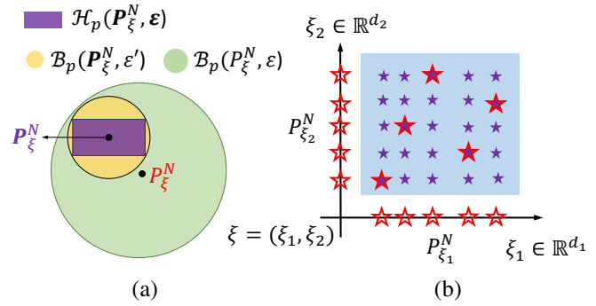
Fig. 2. (a) shows the Wasserstein hyperrectangle \mathcal{H}_p(P_\xi^N, \varepsilon) , its enclosing ball \mathcal{B}_p(P_\xi^N, \varepsilon') around the product empirical distribution P_\xi^N , and the monolithic Wasserstein ball around the empirical distribution P_\xi^N for a random variable with two components. (b) depicts the empirical distribution P_\xi^N from (a) with the filled red stars, which correspond to the N samples, and the product empirical distribution P_\xi^N with the N^2 purple stars. The purple stars are formed by taking the product of the marginal empirical distributions P_{\xi_1}^N and P_{\xi_2}^N of the independent components of \xi , depicted by the hollow red stars.
