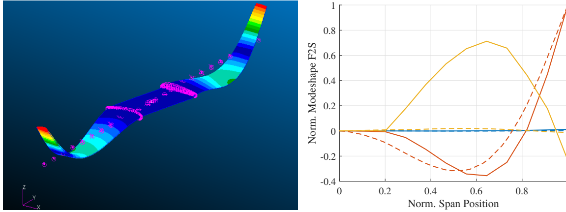
Figure 12 Modeshape F2S
