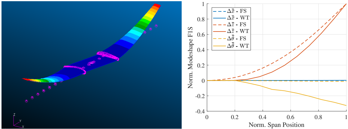
Figure 11 Modeshape F1S
