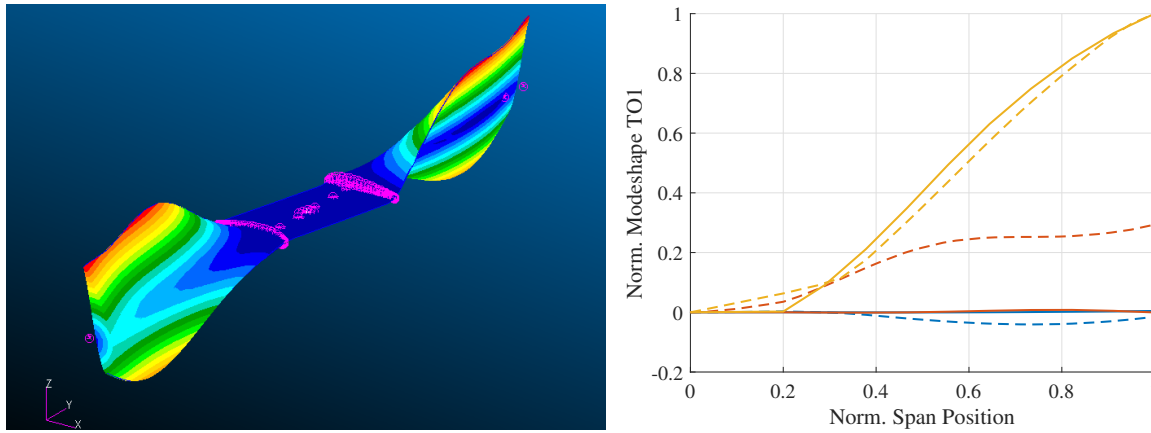
Figure 13 Modeshape TO1
