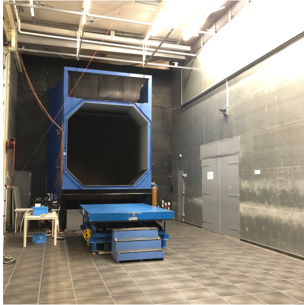
Fig. 7 The Open Jet Facility (OJF) of the Aerospace Engineering faculty at the Delft University of Technology. The OJF has a test section (i.e. nozzle) of 2.85 by 2.85 m and is capable of achieving wind-speeds of up to 35 \text{ m s}^{-1} .
