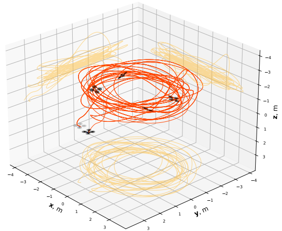
(b) Circular flight trajectory flown in the CyberZoo to achieve velocities of up to 5 \text{ m s}^{-1} .
