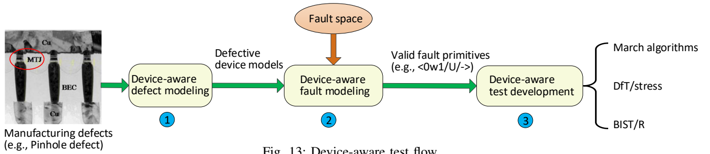
Fig. 13: Device-aware test flow.
