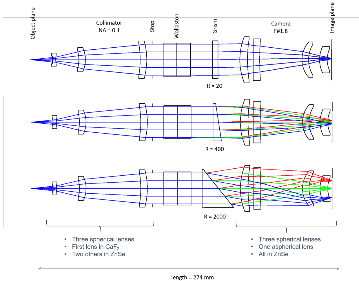
Figure 3: Side view (cut) of the spectrometer optical layout. Each spectral resolution ( R = 20 , 400, and 2000) is depicted. Only the three germanium grisms are changed between each configuration (the focal plane is fixed). They will be mounted on a wheel mechanism.
