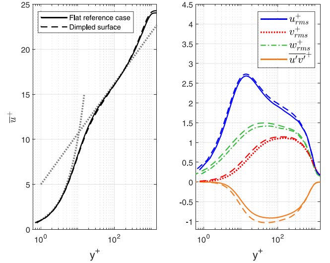
Fig. 14. Boundary layer velocity profiles for the flat reference case versus the dimpled surface (dashed lines) in inner scaling averaged over the region from x/\delta_{99} = 20.4 until 22.5 (which corresponds to the virtual location of 4th center dimple). Left: \bar{u}^+ (black, solid). The gray dotted lines indicate the viscous sublayer, u^+ = y^+ , and the logarithmic region, u^+ = \frac{1}{0.41} \log(y^+) + 5.0 . Right: u^+_{rms} (blue, solid), v^+_{rms} (red, dotted), w^+_{rms} (green, dot-dashed), and u^+v^+ (orange, solid). (For interpretation of the references to color in this figure legend, the reader is referred to the web version of this article.)
