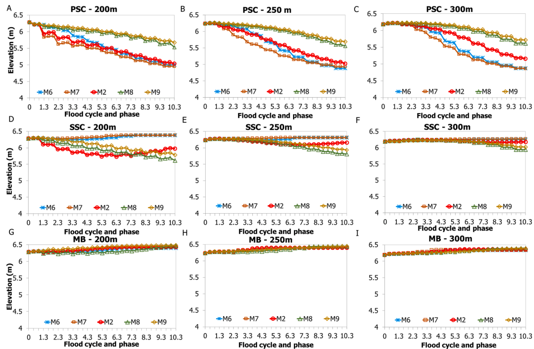
Fig. 9. Elevations of different geomorphological and sedimentary elements for the 10 flood cycles, and the three phases within each cycle, for each of the backflow model runs (M6, M7, M2, M8, M9): PSC: primary splay channel; SSC: secondary splay channel; MB: middle bar. The locations of the floodplain topographic profiles are shown in Fig. 5A. For PSC and SSC, the profile is measured on their lowest points (i.e. bed level) while for middle bar, the profile is measured is on its highest point (i.e. bar top).
