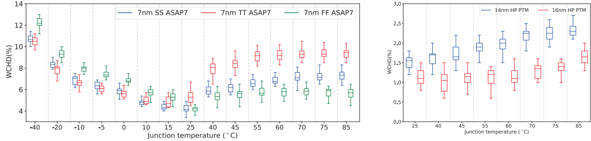
Figure 3: Simulation results - WCHD at different temperatures (a) 7nm ASAP7 (b) 16nm and 14nm HP PTM technology node
