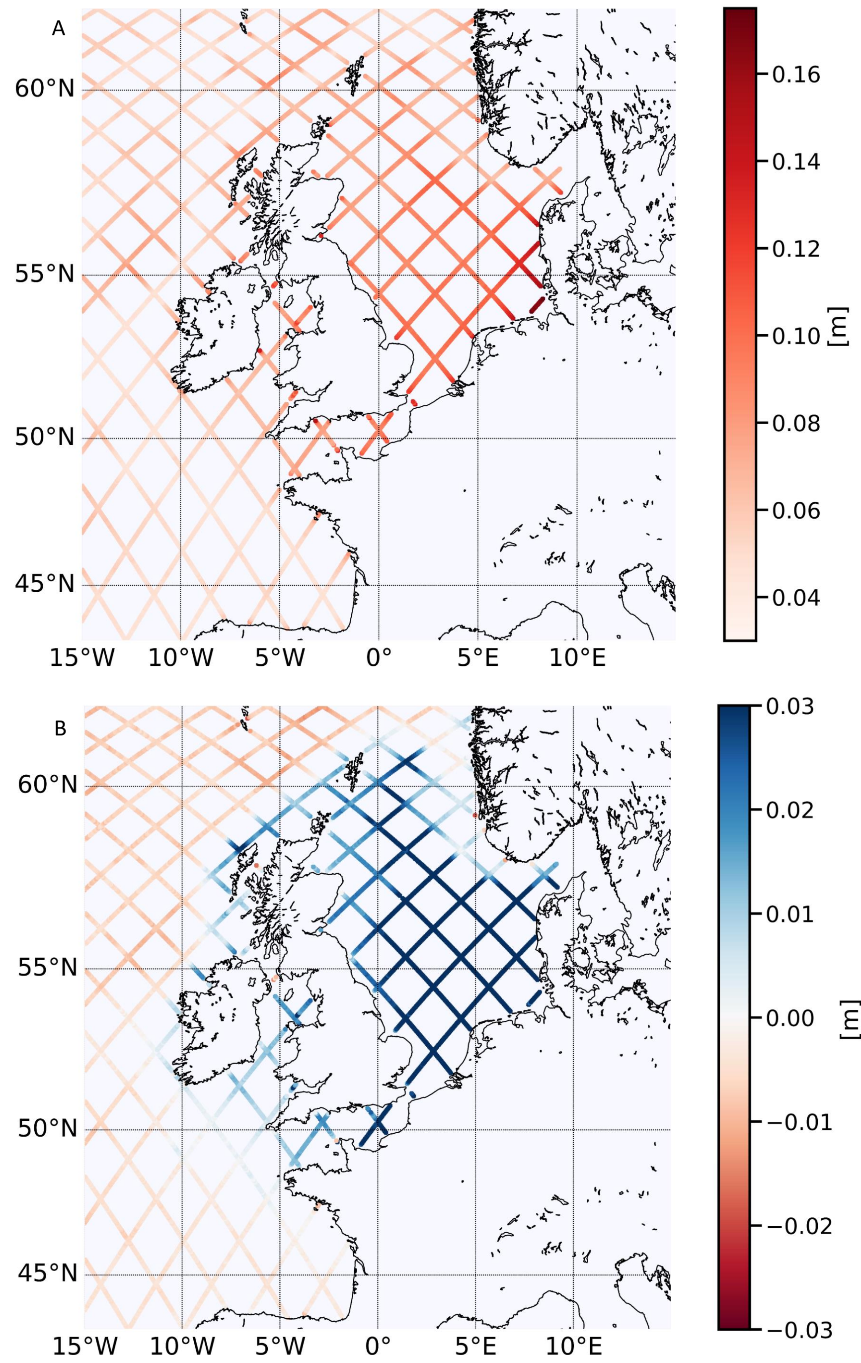
FIGURE 2 - Along track residual standard deviation. A: XTRACK B: XTRACK+DAC – new tidal estimate.
