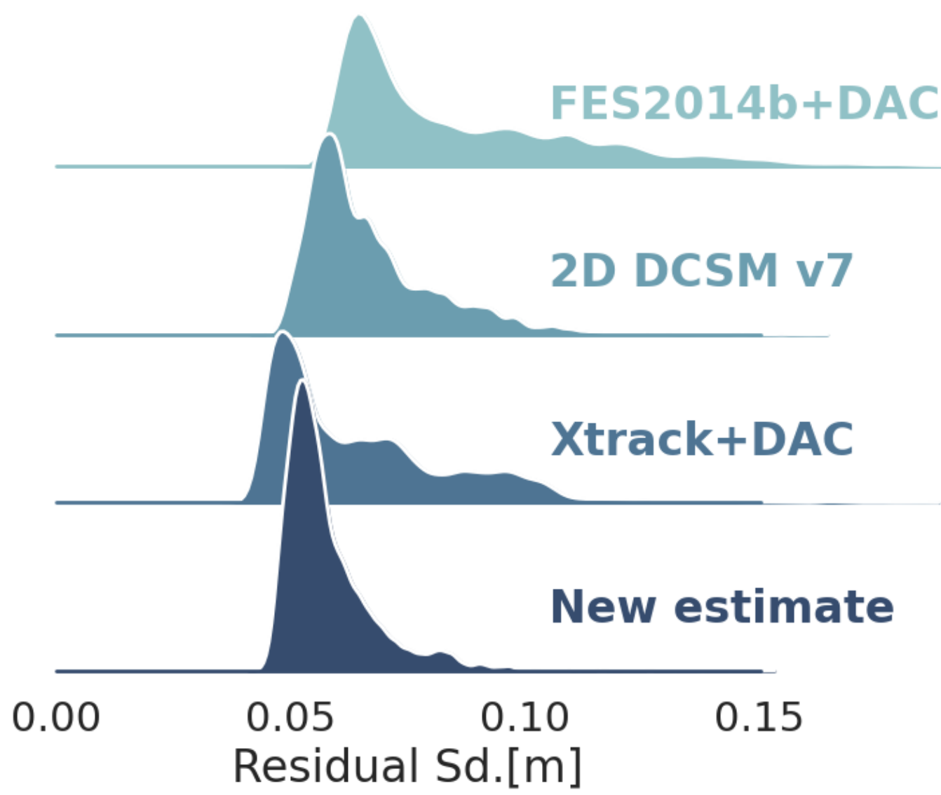
FIGURE 4 – Satellite residual sd. kernel density estimates for the different products.
