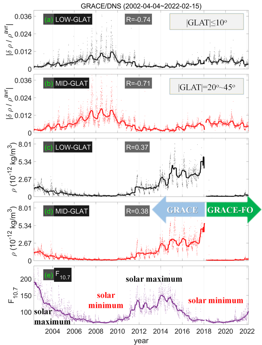
Figure 5. In panels a and b, the small dots represent daily-averaged relative fluctuation amplitude of dayside (07–17 Magnetic Local Time) thermospheric density: (a) low-latitude region ( |GLAT| < 10^\circ ), and (b) mid-latitude region ( |GLAT| = 20^\circ \sim 45^\circ ). Panels c and d are similar to panels a and b, but with the relative fluctuation amplitude replaced by daily averaged \rho . Dots in panel e correspond to the daily F_{10.7} index. The thick curve in each panel is the 160-day (i.e., the time needed for Gravity Recovery and Climate Experiment and GRACE-FO to cover all the local times) moving median of the dots.
