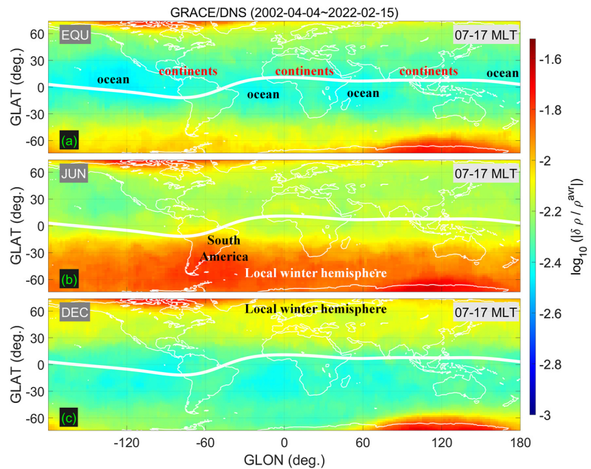
Figure 3. Statistical maps of the relative fluctuation amplitude of thermospheric mass density measured by GRACE(-FO): (a) combined equinoxes, (b) June solstice, and (c) December solstice. The thick white curve represents the dip equator.
