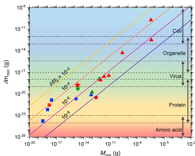
Figure 4. The minimum detectable mass ( \delta m_{\min} ) and the mass of the NEMS resonant mass sensor ( M_{\text{res}} ) determined from literature (square, 1D material; circle, 2D material; triangle, 3D material) and our experiment data (star)
