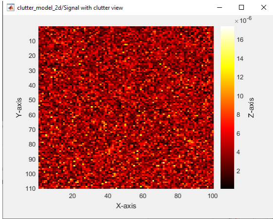
Fig. 7. Sea case. Mixture of clutter and signal. Sea state 5, target RCS 30 m 2 , radar height 2 km, slant range 11.9 km.
