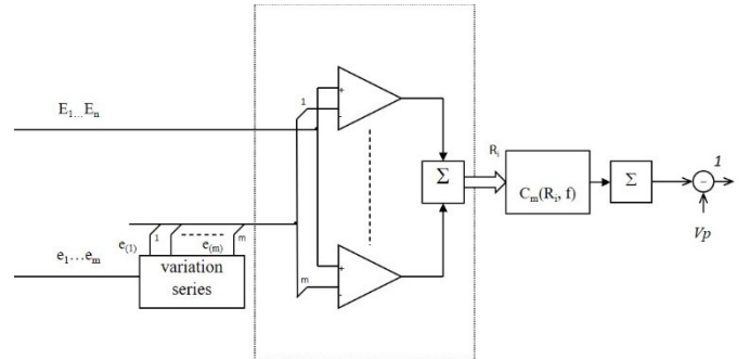
Fig. 4. Structural diagram of a locally optimal rank detector.
