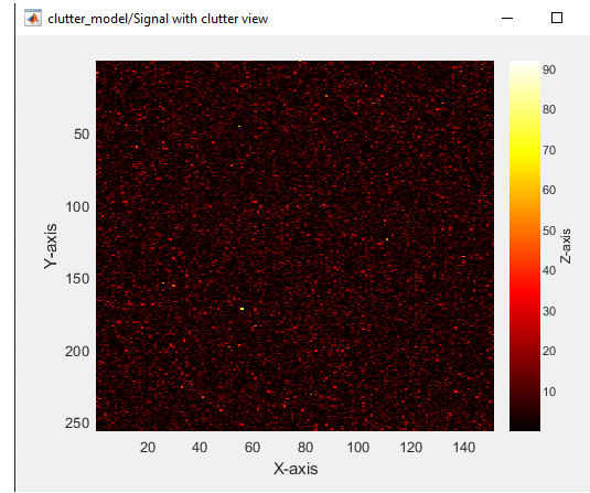
Fig. 9. Rain case. Mixture of clutter and signal. R=10\text{mm/h} , \text{SCR}=-2\text{dB} .
