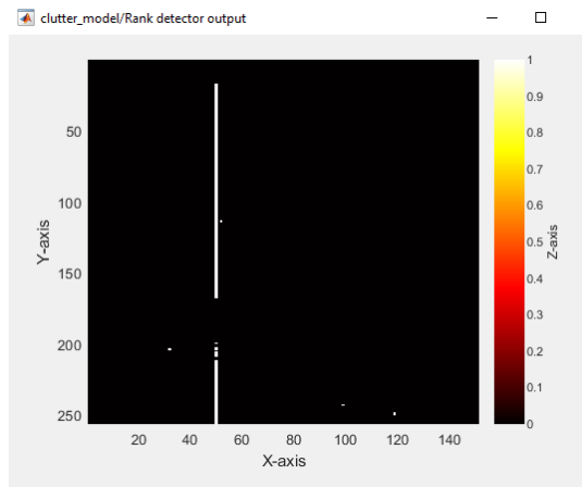
Fig. 10. Rain case. Mixture of clutter and signal. R=10\text{mm/h} , \text{SNR}=-2\text{dB} , N=64 . Clutter suppression result.
