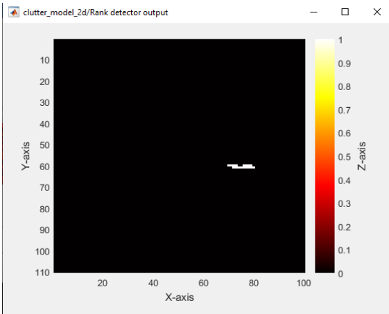
Fig. 8. Sea case. Mixture of clutter and signal. Sea state 5, target RCS 30 m 2 , radar height 2 km, slant range 11.9 km. Clutter suppression result.
