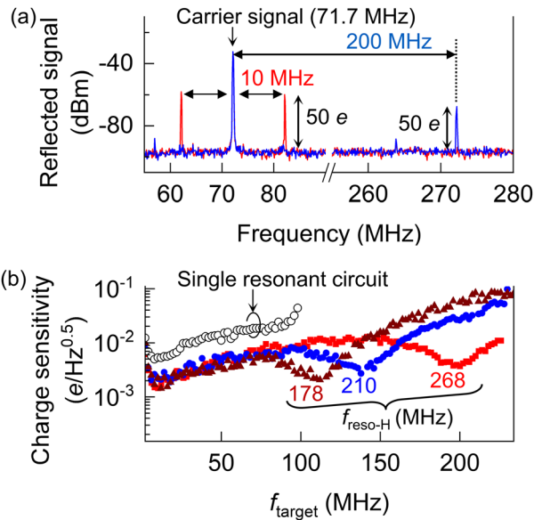
FIG. 3. (a) Detection of the target signal with the reflectometry technique. Frequencies of the target signal are 10 (red) and 200 MHz (blue). The frequency and power of the carrier signal are 71.7 MHz and 10 dBm. f_{\text{reso-L}} and f_{\text{reso-H}} are 72 and 268 MHz. The resolution bandwidth of the spectrum analyzer is 100 kHz. The carrier signal is applied through a coupler, and the reflected signal is monitored with a spectrum analyzer (Rohde & Schwarz FSL). The signal generator for the carrier and target signals is a Rohde & Schwarz SMB 100A. (b) Charge sensitivity characteristics as a function of f_{\text{target}} when f_{\text{reso-L}} and f_{\text{reso-H}} are tuned by C_{\text{Var}} . The characteristics when a single resonant circuit composed of one inductor and C_{\text{stray}} is connected to the sense-FET are also shown. In (a) and (b), L and C_{\text{stray}} are the same as the ones in Fig. 2. The voltage applied to the top gate and word line is 2 V.
