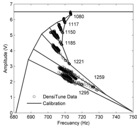
Figure 2. A typical density calibration domain; numbers on the graph are in \text{kg.m}^{-3} (ref: Pedocchi et al., 2015).
