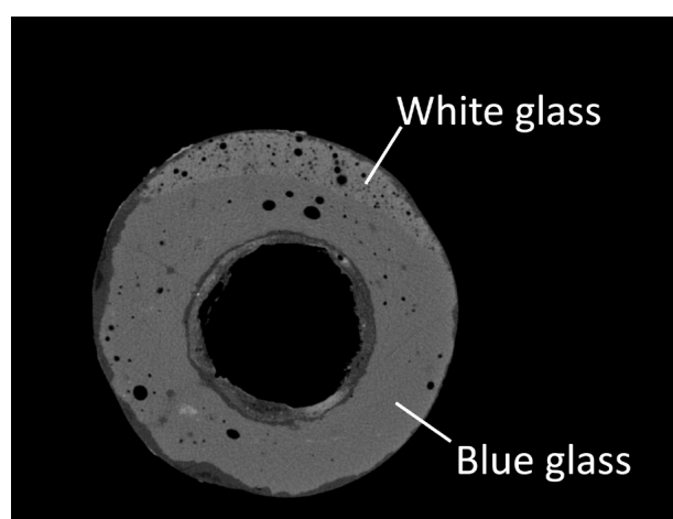
Figure 6. Horizontal X-ray \mu -CT cross section of object 9377 showing more air bubbles in the white glass as compared to the blue glass
