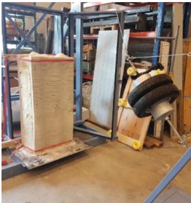
Fig. 6.19 Impact test (Bos et al. 2019)
