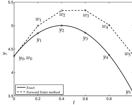
Figure 6.3: Approximation of solution using the Forward Euler method.
