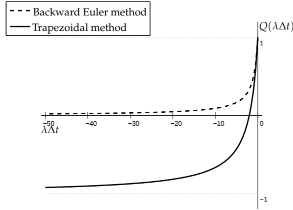
Figure 6.6: Amplification factors of the Backward Euler and Trapezoidal method.
