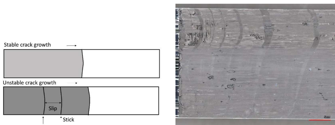
Figure 4. Slip-stick damage propagation (a) schematic of the fracture surface; (b) micrograph of failure surface from 1%CNT200μDCB with slip-stick striations
