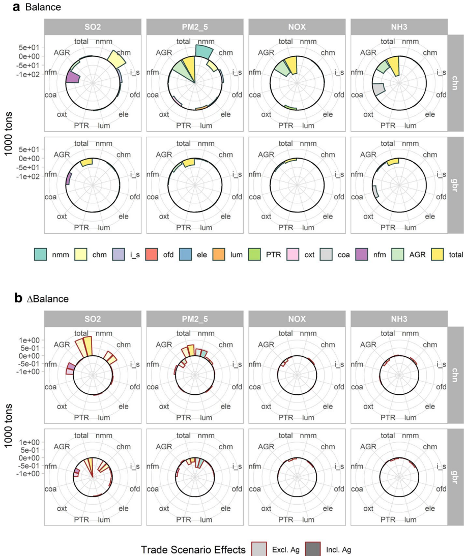
Fig. 3 Air pollution embodied in balance of trade (a) and the changes under China-UK FTA scenarios (b) by sector Notes: PM2_5=PM2.5, nmm=non-metallic mineral products, chm=chemical products, i_s=ferrous metals, ofd=food products (nec), ele=electronics, lum=wood products, PTR=oil and gas, oxt=minerals (nec), coa=coal, nfm=metals (nec), AGR=agriculture, total=all, where nec means “not elsewhere classified.” See Tables s1 and s5 in Online Resource 1 for more details on sector definition and aggregation. Panel a shows the values for China (chn) and the UK (gbr) under Default, while panel b exhibits the changes with respect to baselines. To save space and for clarity, only the sectors with magnitudes (in balance) > 3% of the maximum sectoral magnitude (for both China and the UK) are presented here
