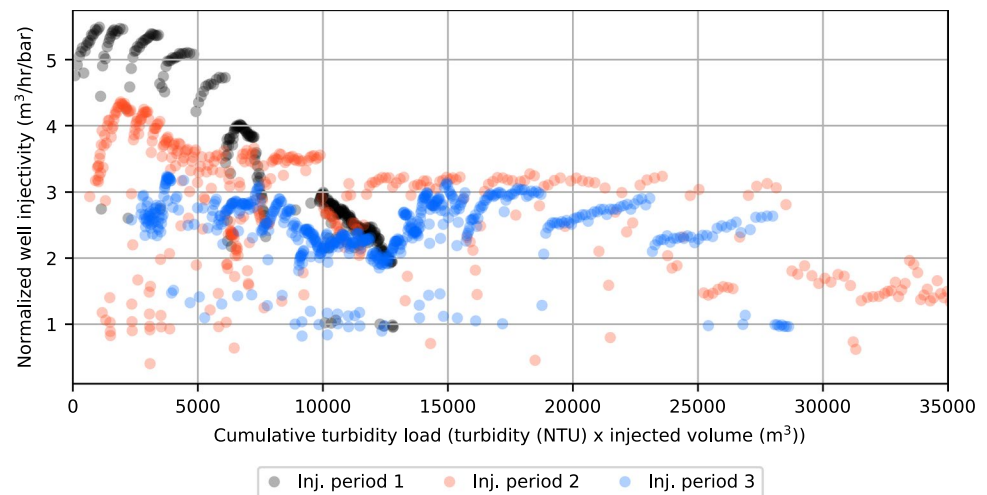
Fig. 7 Overview of the normalized well injectivity versus the cumulative turbidity load—turbidity (NTU) \times injected volume ( \text{m}^3 )—during the three injection periods
