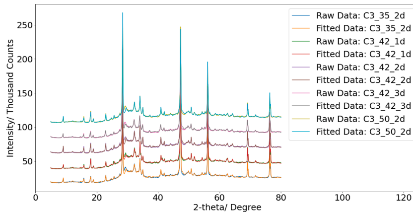
Fig. 12. XRD pattern and Rietveld refinement.
