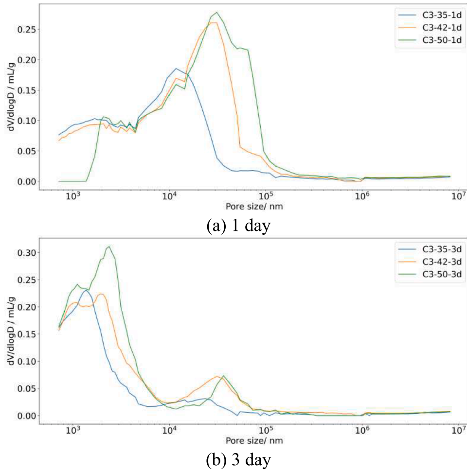
Fig. 14. Pore size distribution derived from MIP results.
