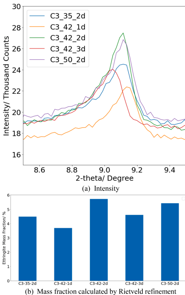
Fig. 13. Ettringite content measured by XRD.
