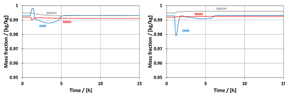
Fig. 9 – Mass fraction in the product streams of the MMH plant during 20% production rate increase (left) or decrease (right).
