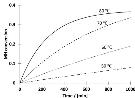
Fig. 3 – Left: figure with experimental data reported in literature (Karinén and Krause, 1999); Right: calculated MH conversion, initial ratio MeOH:MH = 2, inert mole fraction 0.7, catalyst concentration 0.0125 g/cm 3 , reaction rate given by Eq. (13).
