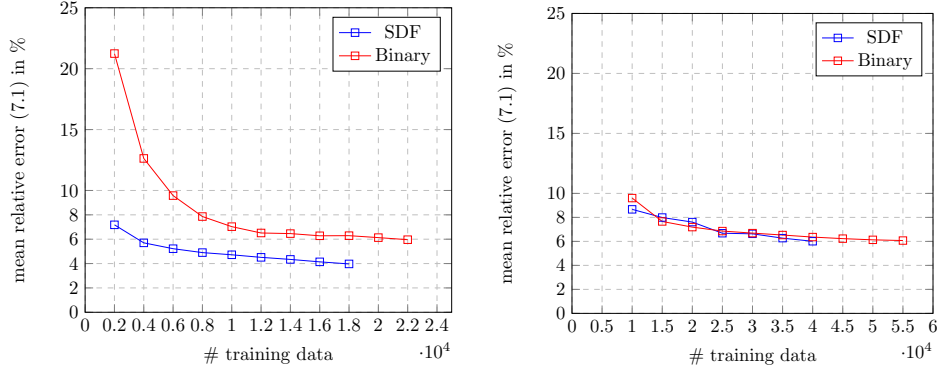
FIG. 9.1. Mean relative error (7.1) for our sequential learning strategy as described in Section 9: results for type I–III data (left) and for type IV data (right).
