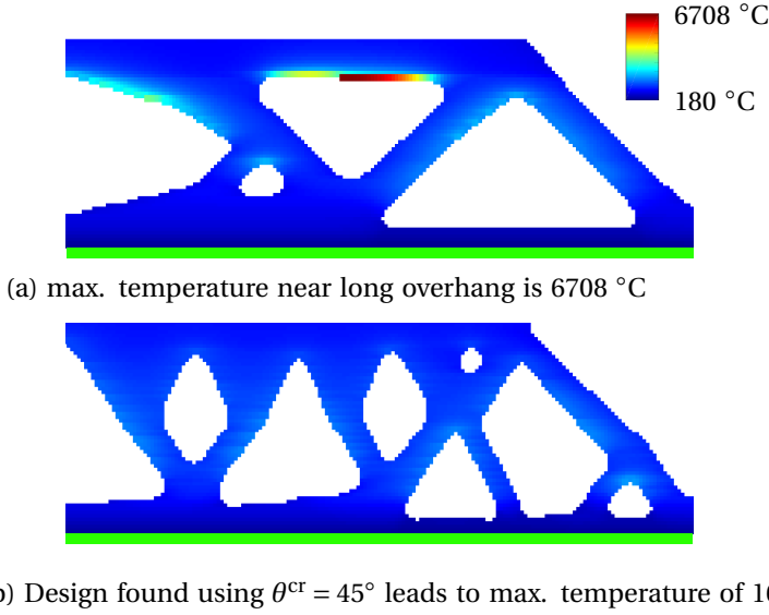
Figure 4.9: Hotspot map obtained from high-fidelity LPBF transient simulation for designs found using (a) Robust TO without the hotspot constraint (b) Robust TO with the hotspot constraint. The high-fidelity transient simulation considers temperature dependent thermal properties, convection and radiation and all simulation parameters are taken from Ranjan et al. [35].
