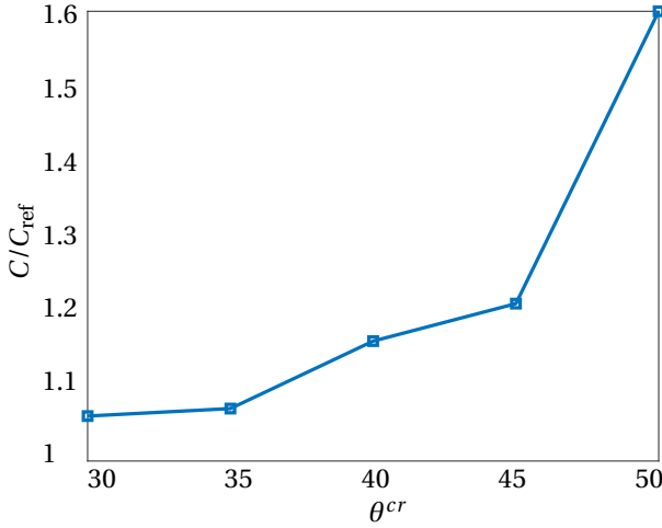
Figure 4.11: The variation of compliance with respect to the overhang angles used for defining the critical hotspot temperatures. The compliances are normalized against that for the reference design shown in Figure 4.8a.
