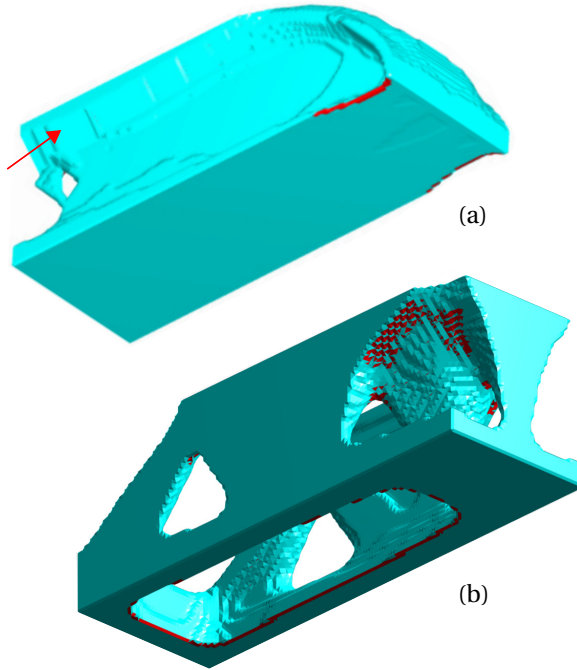
Figure 5.18: STL facets which have overhang angles less than \theta^{\text{cr}} = 45^\circ are marked red for (a) AM-filter and (b) HS 45 designs.
