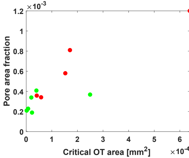
Figure 5.17: The variation of pore area fraction with respect to respective critical OT area \overline{OT} . It is evident that \overline{OT} values for HS 45 cross-sections remain on the lower side resulting in lower pore formation as compared to the AM-filter design.
