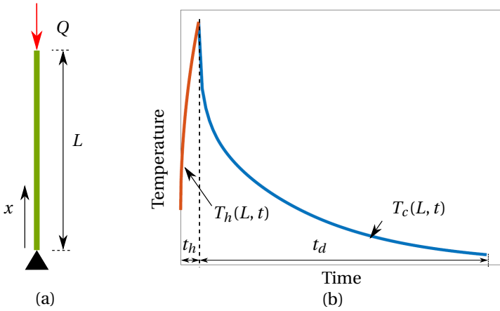
Figure 3.7: (a) one-dimensional domain with length L subjected to boundary conditions reminiscent to the reference model, i.e., heat flux Q acts at x=L while bottom temperature is fixed at T=T_s . (b) Thermal history of the topmost point ( x=L ) of the rod during a heating and cooling cycle.
