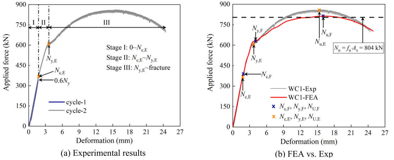
Fig. 16. Load-displacement curves of WC1.
