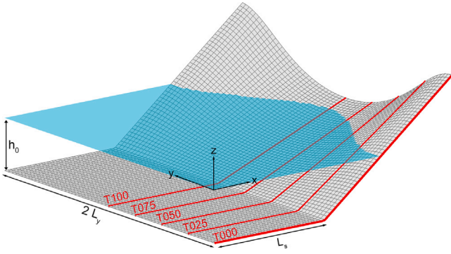
Fig. 2. Problem geometry Zelt test case. L_y is the half wavelength of the sinusoidal bay; L_s is the width of the shelf; T_{xxx} indicates the number of the line where the run-up heights are recorded in Fig. 3(a).
