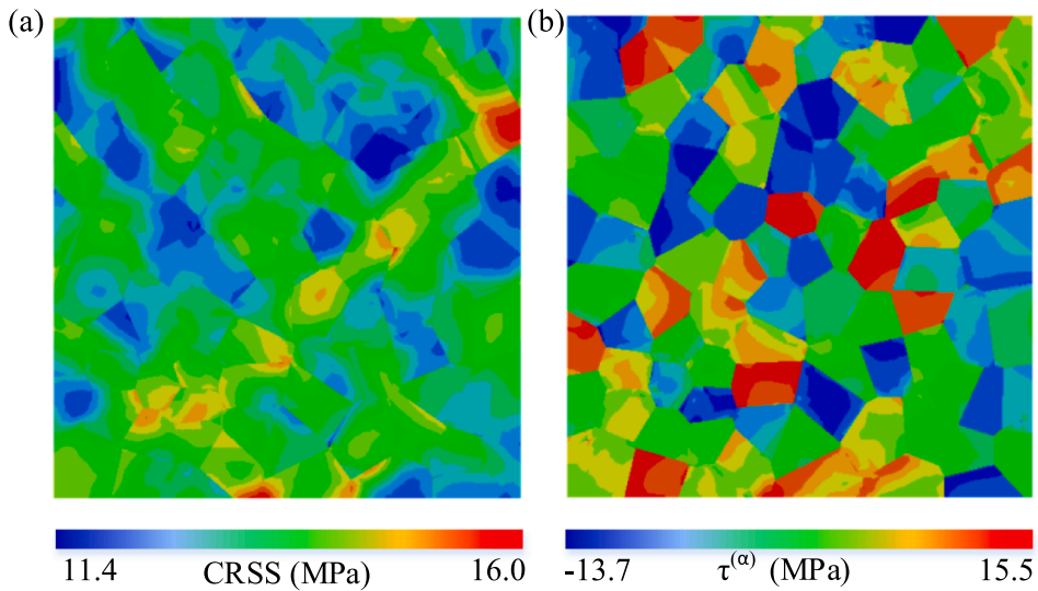
Fig. 5. Distributions of CRSS and \tau^{(a)} of the \{111\} \langle 0-11 \rangle slip system for sintered AgNP at -40 \text{ }^{\circ}\text{C} and strain rate of 10^{-5} \text{ s}^{-1} : (a) CRSS; and (b) \tau^{(a)} .
