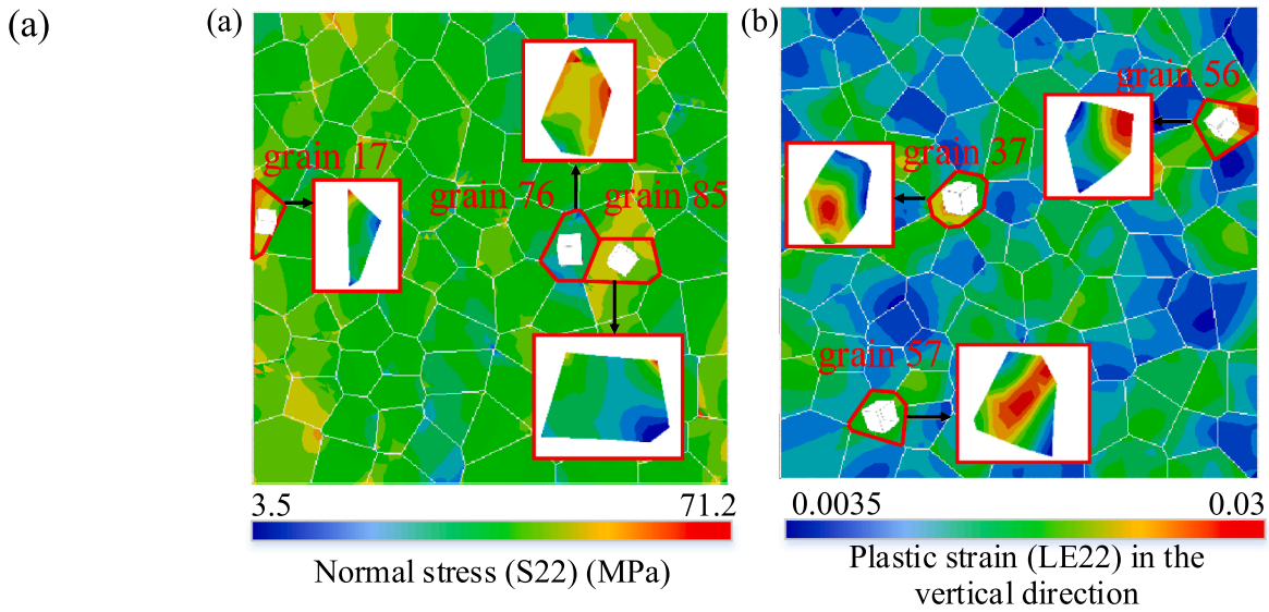
Fig. 9. Stress and strain contours in the polycrystal structure at -40^\circ\text{C} and the strain rate of 10^{-4}\text{ s}^{-1} : (a) normal stress (S22); and (b) plastic strain (LE22) in the vertical direction.
