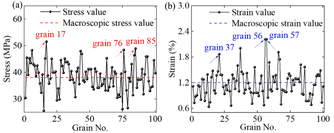
Fig. 10. Stress and strain values of individual grains at -40^{\circ}\text{C} and the strain rate of 10^{-4}\text{ s}^{-1} : (a) normal stress (S22); and (b) plastic strain (LE22) in the vertical direction.
