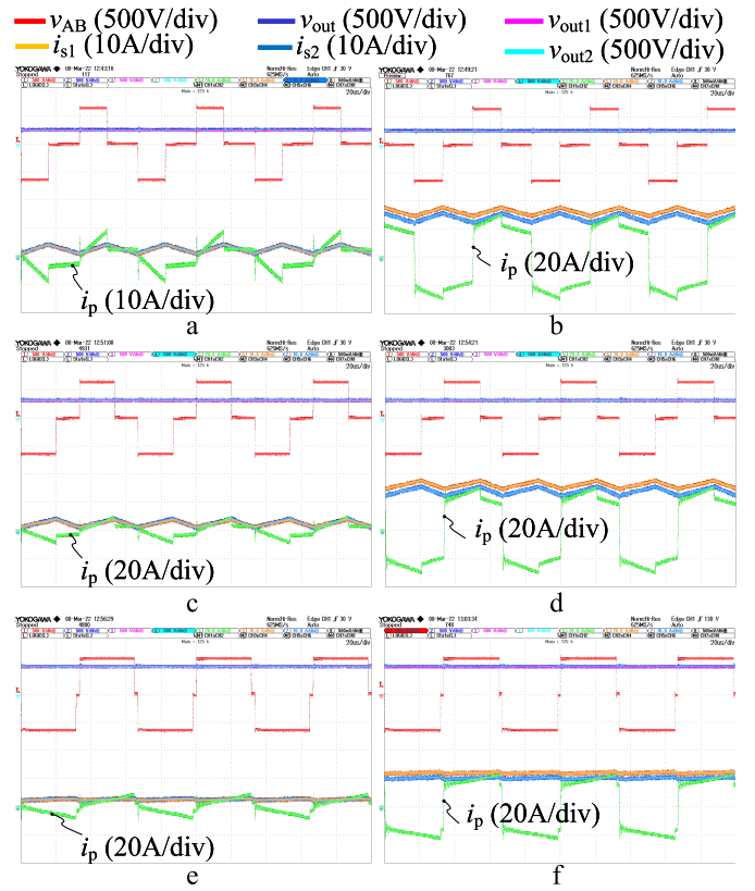
Fig. 10. Operational waveform of the r-PSFB converter in the parallel connection mode with V_{in} = 640 V. v_{out1/2} and i_{s1/2} are the output voltage and current of the two secondary side rectifiers, measured after the RCD circuitry and on the output inductors, respectively. (a) V_{out} = 250 V, I_{out} = 5 A. (b) V_{out} = 250 V, I_{out} = 30 A. (c) V_{out} = 320 V, I_{out} = 5 A. (d) V_{out} = 320 V, I_{out} = 30 A. (e) V_{out} = 500 V, I_{out} = 5 A. (f) V_{out} = 500 V, I_{out} = 22 A.
