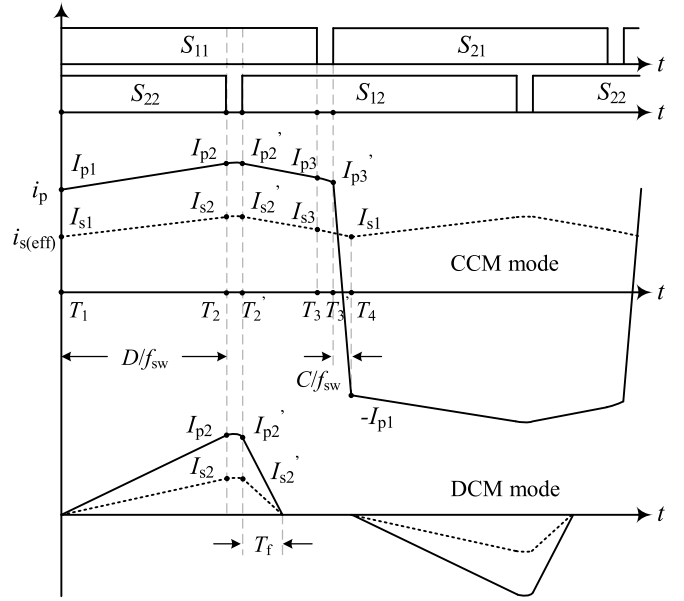
Fig. 4. Typical switching signals and current waveform of the PSFB converter in CCM and DCM.
