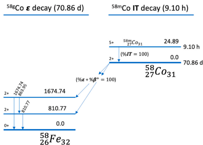
Fig. 1. Decay scheme of ^{58\text{m}}\text{Co} into the stable ^{58}\text{Fe} . Data from (IAEA Nuclear Data Section, 2021).
