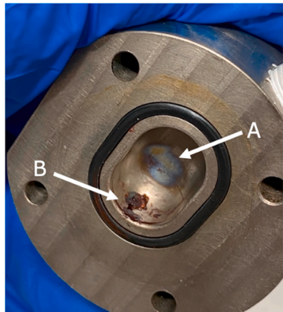
Fig. 6. Picture of the target chamber opened up for maintenance showing blueish colored stain in the back of the chamber (A) and brownish iron sludge in the bottom (B).
