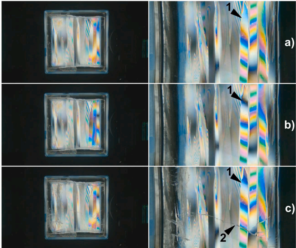
Fig. 7. Global straight and oblique close-up video views from Test #2 with frames a) prior to loading; b) initial loading, just before fracture; and c) immediately after fracture. Indicator 1 points to the same location in each frame, highlighting the change in the shape and color of the interference color pattern in the grain with loading. Indicator 2 points to a large crack which unloaded the grain (compare Indicator 1 in b) and c)).
