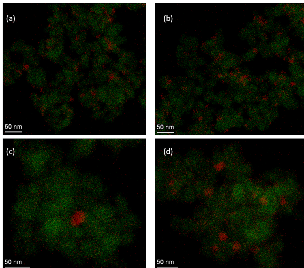
Fig. 8. EDX mappings of (a–b) a reduced and passivated and (c–d) a used Co(4)/TiO 2 catalyst: the cobalt mapping is shown in red and the titania mapping in dark green. (For interpretation of the references to colour in this figure legend, the reader is referred to the web version of this article.)
