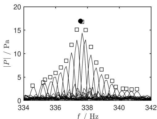
Figure 3. Fourier transforms of the recordings for the estimation of the resonance frequency in D_6 at a 255 kPa and 629.8 K: □, maxima of each individual Fourier transform (amplitude is divided by 3); ●, maximum of the resonance peak (amplitude divided by 3).
