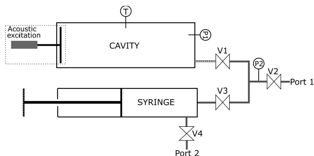
Figure 1. General layout of the OVAR setup.
