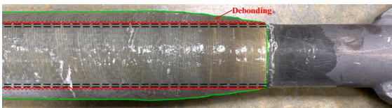
c) HSS joint with lowest resistance failing due to full debonding
