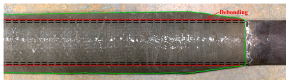
a) MS joints fails at the steel-composite bonded interface (full debonding)
