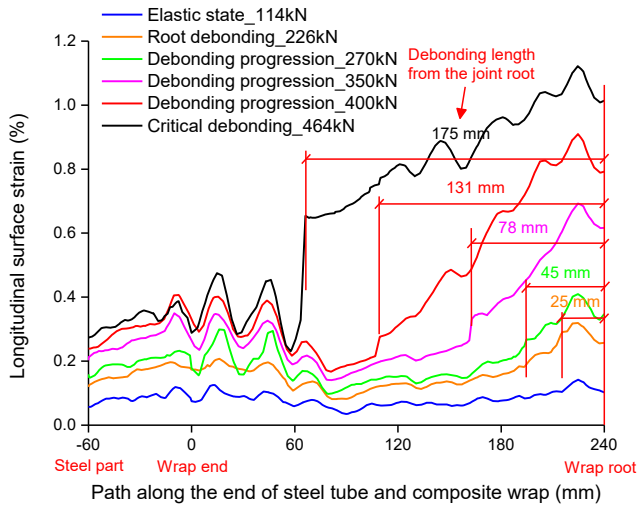
a) Strains at characteristic loading states corresponding to progression of failure
