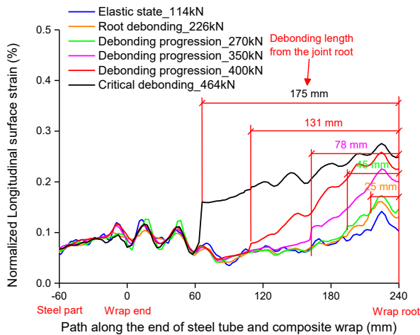
b) Strains normalized to load level corresponding to the elastic state (114 kN)
