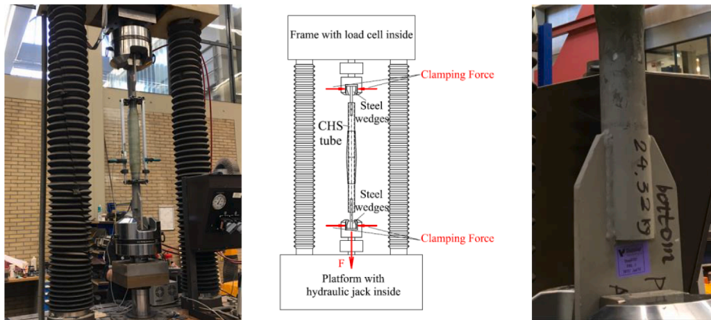
a) Experimental set-up configuration b) Schematic experimental set-up c) Load introduction at the brace end
