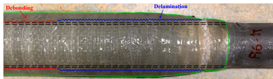
b) HSS joints failing due to combined debonding and delamination
