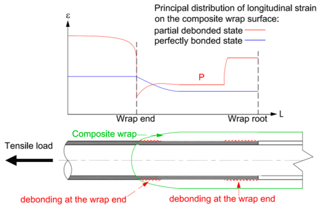
Fig. 12. Principle of using variation of the distribution of longitudinal surface strains on composite wrap to determine debonding crack length in the embedded bonded interface.
