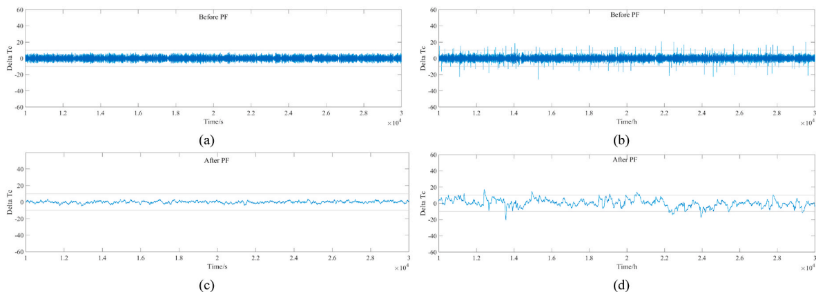
Fig. 11. Residual values of \Delta T_C with and without cooling system degradation, (a) without degradation before PF (particle filtering), (b) with degradation before PF (particle filtering), (c) without degradation after PF (particle filtering), and (d) with degradation after PF (particle filtering).
