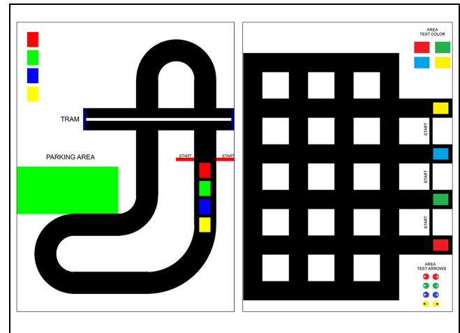
Figure 1. Network layouts for the Automated Vehicle Traffic Challenge competition. On the left the J-shaped track corresponds to highway conditions. On the right the #-shape track corresponds to urban conditions.
