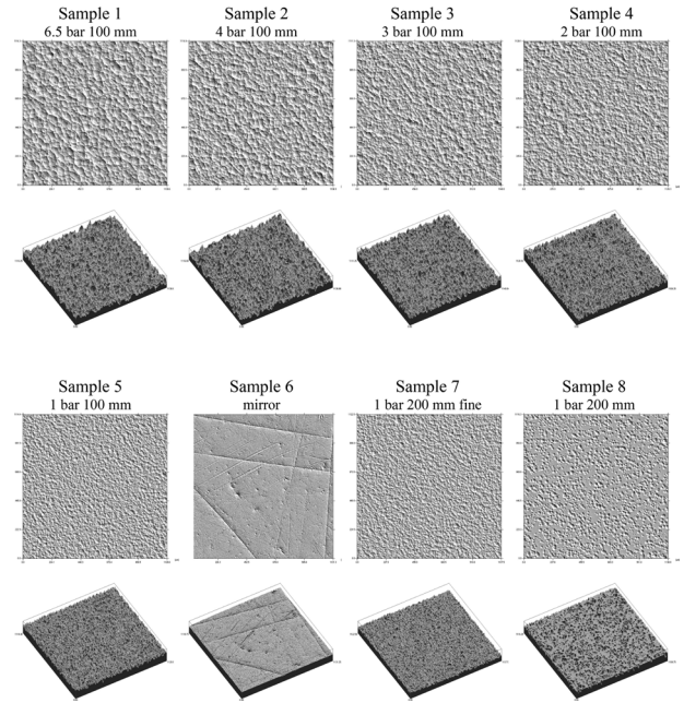
Figure 2: Top and 3D views of the samples' surface topographies measured with a confocal microscope. Except for Sample 6, the surfaces consist of randomly distributed holes caused by the glass beads of the sandblaster.
