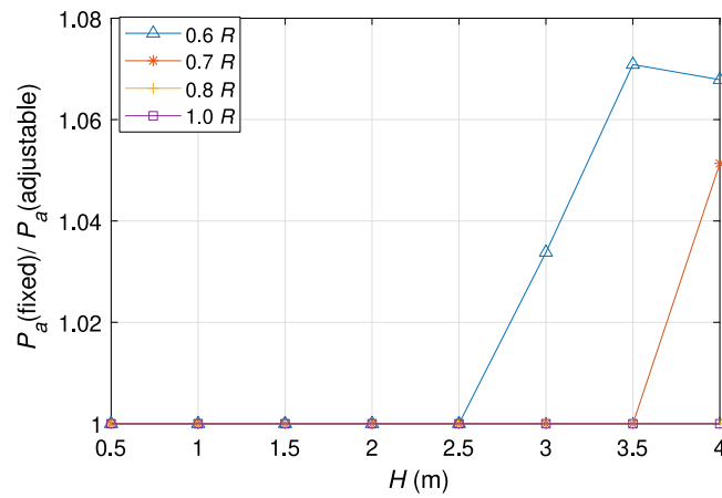
Fig. 11. The average absorbed power of the fixed draft WEC with the draft of 3.5 m normalized to that of the adjustable draft WEC with the draft of 3.5 m, and B_{po} = 30 kNs/m and T = 7.0 s. The considered motion limits range from 0.6R to 1.0R .
