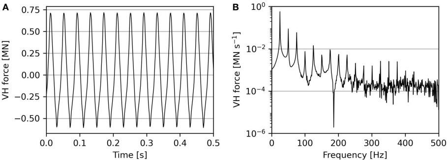
FIGURE 4 Estimated vibratory force exerted by the installation tool at the pile head as a function. (A) shows the time signature and (B) the amplitude spectrum of the force (Tsetas et al., 2023a).
