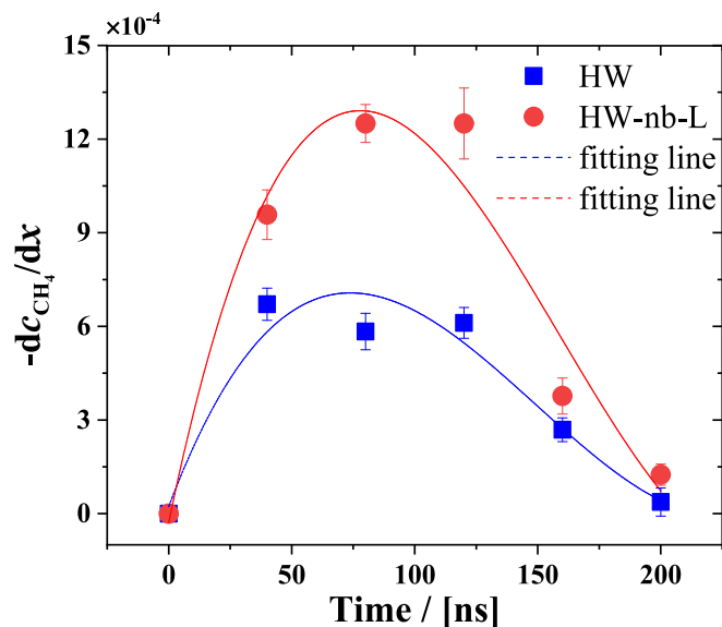
Fig. 10. Negative derivatives of the methane concentration in the liquid phase along the X-axis. The distance (x) is taken from the residual hydrate surface to the central position of the bulk phase and from the center of area 1 to the bulk-phase center after the hydrate dissociated in the HW system. The calculation distance is from the hydrate surface to the pre-existing surface and from the center of area 1 to the bubble surface after the hydrate dissociated. The lines are third order polynomials. The coefficients of determination R^2 are equal to 0.9405 and 0.9488 for the HW and HW-nb-L systems, respectively.
