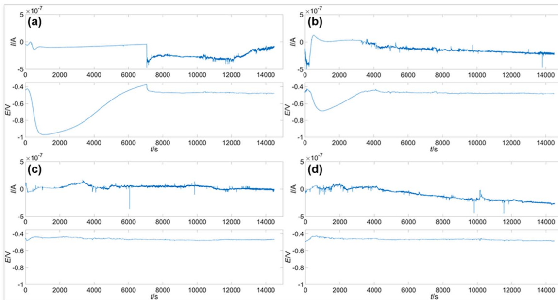
Figure 2. EN current (top) and potential (bottom) signals for AA2024-T3 initially treated in 0.01 M NaCl and 0.01 M Li 2 CO 3 solution for 14500 s (approximately 4 h), and then exposed in 0.01 M NaCl after ambient ageing for (a) 0 h, (b) 4 h, (c) 24 h, and (d) 72 h.
