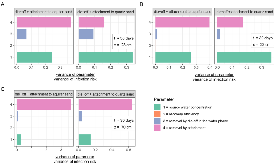
▲ Figure 6 Sensitivity analysis to analyze the impact of parameters on the infection risk. A-C: Analysis of different ASTR operations as described in the box on the right side of each graph. Left panel always analyses ASTR with pathogen removal by die-off in the water phase and attachment aquifer sand, right panel analyses ASTR with pathogen removal by die-off in the water phase and attachment quartz sand. Scenario 1-4 relate to the different input parameters that impact the final infection risk. The value of the ratios is irrelevant but allows to compare the different parameters with each other.
