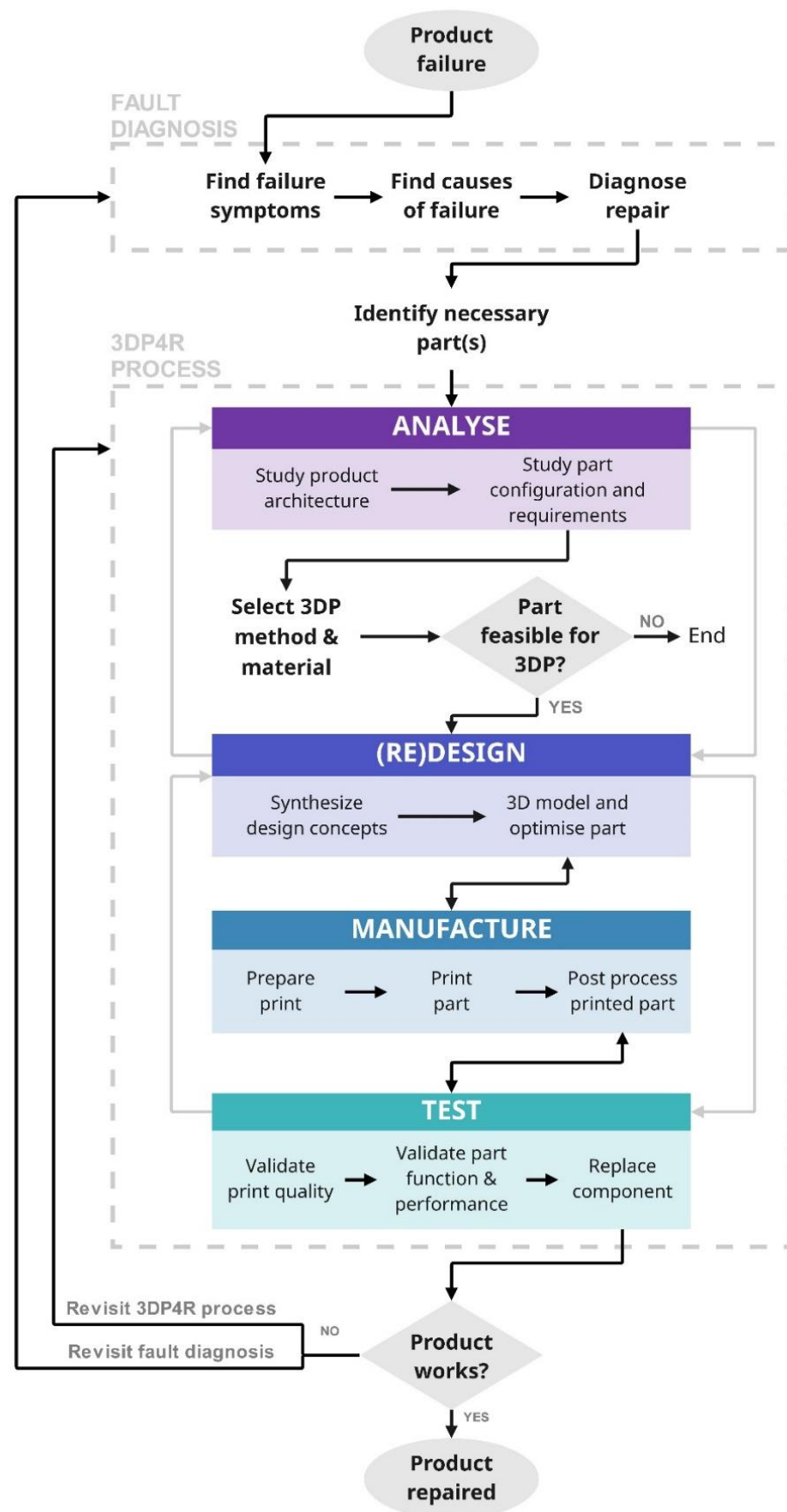
Figure 12. 3DPfR framework.
