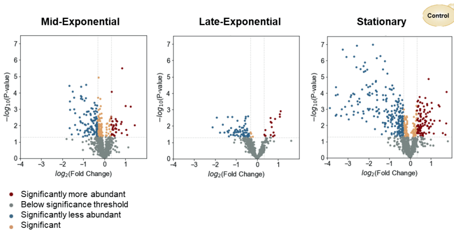
SI Figure 4. Global proteome changes between aerobically and anaerobically cultured CEN.PK113-7D yeast cells. The \log_2 of the abundance fold change between the two conditions (normalised to the aerobic experiments) was plotted against the -\log_{10} of the p-value. The mid-exponential (ME), late-exponential (LE) and mid-stationary (MS) phases were compared. P-value threshold < 0.05 , fold change threshold > 1.5 ( \log_2 fold change threshold \pm 0.32 ).
