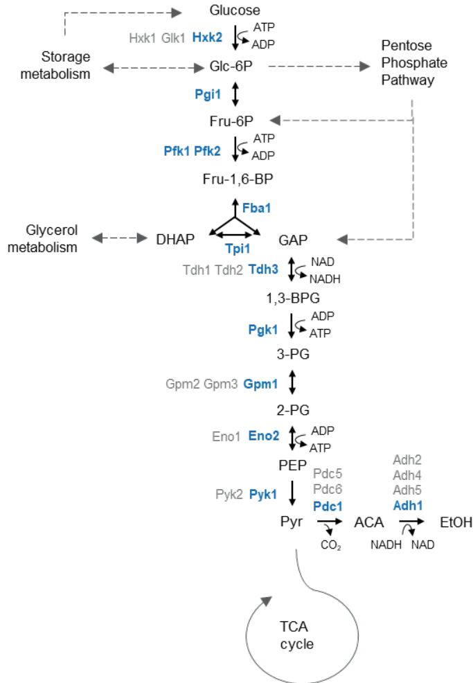
Figure 3. Schematic overview of S. cerevisiae glycolysis and associated pathways in the central carbon metabolism. The graphs outlines the major (blue) and minor (grey) S. cerevisiae isoenzymes. Only the major isoenzymes are retained in the minimal glycolysis strain.
