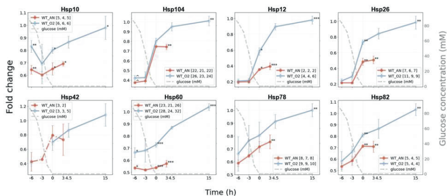
SI Figure 5. Fold changes (FC) of heat shock proteins from CEN.PK113-7D under aerobic and anaerobic conditions. The biological-replicate-averaged FCs were plotted against the time relative to glucose depletion (0h) in hours. Orange: CEN.PK113-7D under anaerobic conditions, light blue CEN.PK113-7D under aerobic conditions. The error bars show the standard deviation of the mean of the three biological replicates. In the legend, the numbers between brackets represent the number of unique peptides that were found in each biological replicate. The grey dashed line represents the glucose concentration in time in millimolar (mM), shown on the secondary y-axis. Asterisks (*) and circumflexes (ˆ) indicate the significance between the aerobic and anaerobic experiments. Different p-values were indicated: < 0.001 (***), < 0.01 (**), < 0.05 (*), and < 0.1 (ˆ).
