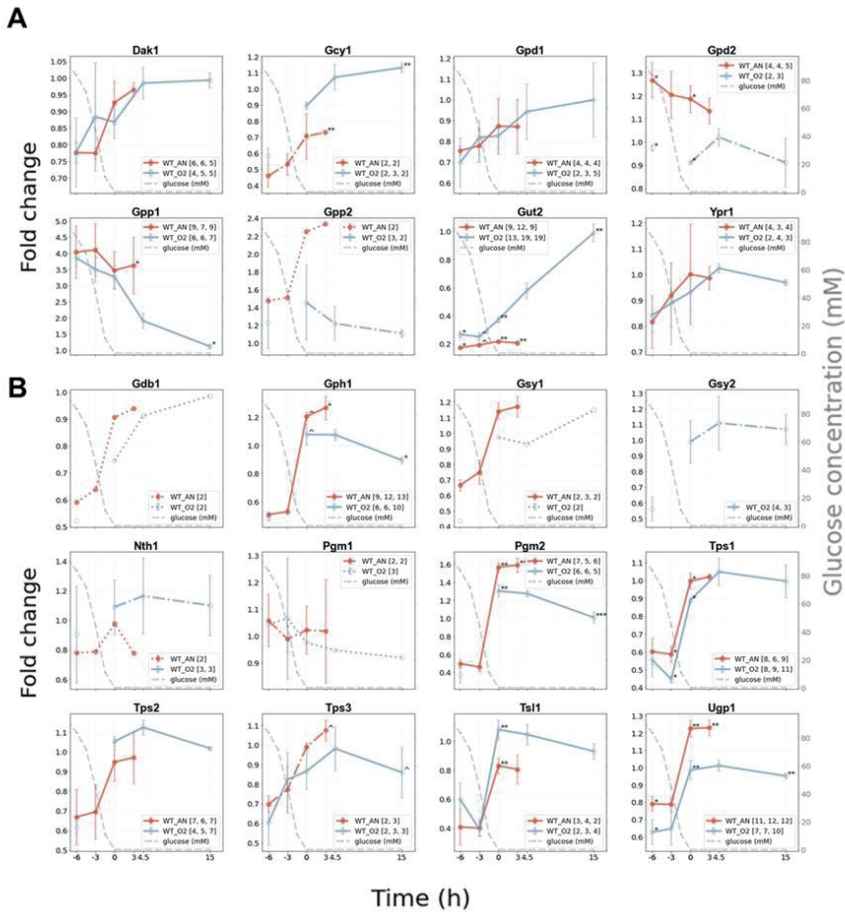
SI Figure 3. Protein profiles of CEN.PK113-7D in glycerol, glycogen and trehalose metabolism during aerobic and anaerobic growth. The biological-replicate-averaged fold-change values were plotted against the time relative to glucose depletion in hours for proteins involved in glycerol (A) and glycogen and trehalose (B) metabolism. The different colours of the line graphs represent: orange the control strain under anaerobic conditions (WT_AN), light blue: the control strain under aerobic conditions (WT_O2). The error bars show the standard deviation of the mean of the three biological replicates. The grey dashed line represents the glucose concentration in time in millimolar (mM), shown on the secondary y-axis. The number of quantified peptides per biological replicate are given in brackets. Asterisks (*) and circumflexes (ˆ) indicate the significance between the aerobic and anaerobic experiments. P-values are indicated as follows: < 0.001 (***), < 0.01 (**), < 0.05 (*), and < 0.1 (ˆ).
