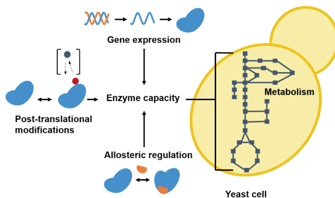
Figure 1. Overview of metabolic regulation mechanisms in a yeast cell. The metabolic flux in cell depends on the capacities of the metabolic enzymes, which depend on enzyme abundances, allosteric regulation but also on the occurrence of covalent modifications on the protein itself, termed post-translational modifications (PTMs).
