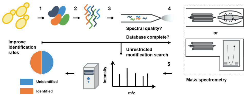
Figure 2. Protein identification by (a bottom-up) shot-gun proteomics experiment. The typical workflow consists of cell lysis, protein extraction from (yeast) cells and subsequent digestion into peptides using specific proteases (step 2). In step 3, the peptides are separated by liquid chromatography and further detected following electrospray ionization (ESI) by data dependent analysis, which automatically collects fragmentation spectra from (top intense) peptide signals, in step 4. In step 5, the fragmentation spectra (MS/MS) are commonly identified by database search approaches, matching fragmentation spectra to in-silico peptides derived from the target proteome database. Finally, the result of a typical shotgun proteomics experiment is depicted, in which roughly half of the spectra could not be assigned to a target protein sequence of the database. Similar identification rates have been reported in a survey reinvestigating hundreds of shot-gun proteomics experiments by Griss et al. (2016). To improve the identification rate, several approaches can be taken. First, the quality of the spectra should be verified. In addition, modifications could be added to the database to ensure that the database is complete and modified peptides could be identified. Finally, an unrestricted search could be performed to identify (unexpectedly) modified peptides.
