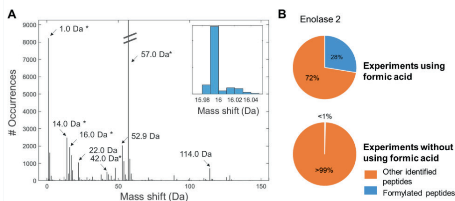
Figure 3. Peptide modification search. A. Unrestricted modification search as obtained by using the Byonic software tool (Table 2). The observed mass shifts (between 0 and 150 Da) on tryptic peptides from a yeast shot-gun proteomics experiment are represented in a histogram. Commonly, many mass additions derive from artificial modifications introduced during sample preparation, while others are of natural origin. However, the distinction between both types is a delicate step during data processing and evaluation. Common mass shifts found are indicated by an arrow: Deamidation (0.98 Da) ^{13}\text{C} isotope precursor selection (1.0 Da), methyl (14.0 Da), oxidation (15.98 Da), sodium adduct (22.0 Da), acetyl (42.0 Da), iron adduct (52.9 Da), carbamidomethyl (57.0 Da) and dicarbamidomethyl or ubiquitin (114.0 Da). Phosphorylation (80.0 Da) was not observed frequently in this search, even though it appears to be the most commonly observed PTM in yeast [189]. However, this modification type usually occurs at low stoichiometry and therefore enrichment methods are commonly applied, which was not performed here. (*) Indicated mass shifts can also represent amino acid substitutions, which require case-by-case investigations. Inset: Assignment of high-resolution mass shifts. Where high-resolution mass spectrometry can resolve 15.99 (oxidation) from a closely related addition at 16.02 Da. Other amino acid substitutions such as Ala→Ser show exactly the same composition and therefore mass shift. B. The degree of formylation of Enolase 2 ( S. cerevisiae ) is quantified following a common shotgun proteomics experimental set-up with or without the use of formic acid as a solvent for protein solubilisation. The use of formic acid during sample handling introduced a considerable number of formylated peptide artefacts, as shown for Enolase 2.
