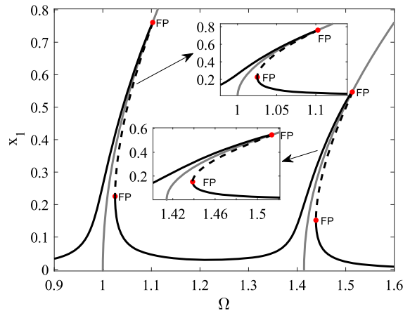
Fig. 8 Frequency response diagram of the two-DOF system without the free-play. The black continuous and dashed curves represent, respectively, the stable and unstable amplitude of the first mass, while the grey curve represents the backbone curves. (Colour version online)
