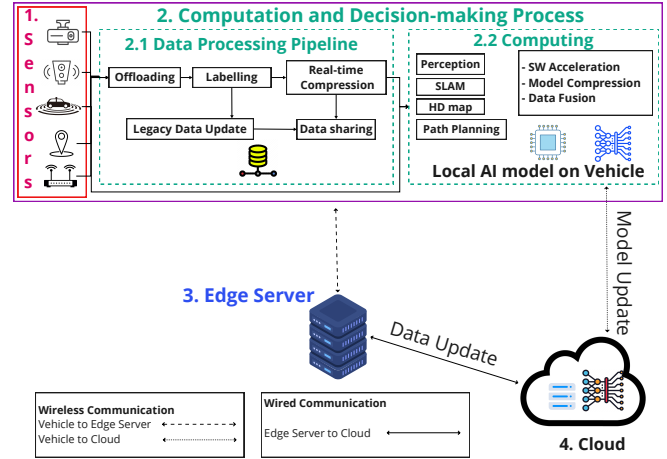
Fig. 6. Edge-AI Pipeline
