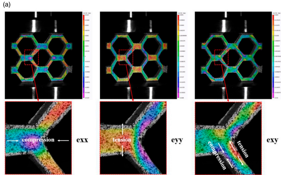
The strain of the sample when the load is applied along the X direction.
