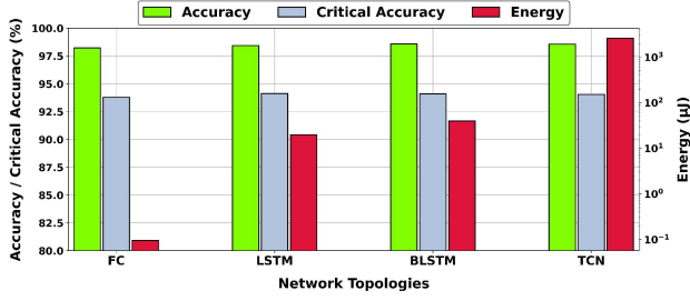
(a) Design space exploration for classifier C1
