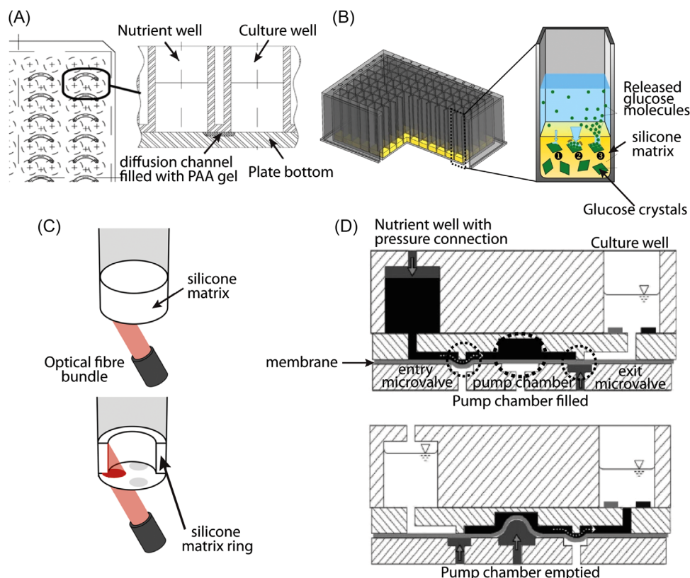
FIGURE 4 Different types of modifications made to conventional microtiter plates to enable fed-batch cultivation. (A) Fed-batch microtiter plate showing a pair of wells connected by a polyacrylamide gel filled microchannel. One well acts as a cultivation chamber and the other as a reservoir for nutrients, with the nutrient supply controlled by the diffusional properties of the gel. Adapted from Wilming et al. [13] (B) Fed-batch microtiter plate with a glucose containing silicone matrix at bottom of each well. Adapted from Keil et al. [14] (C) Adaptation of the concept in (B) from a disc to a glucose-releasing ring, enabling optical accessibility during cultivation. Adapted from Habicher et al. [17] (D) Fed-batch microtiter plate with the bottom replaced by a PDMS microfluidic chip that connects pairs of wells (microfluidic Biolector). Precise delivery of nutrients from the nutrient well to the culture well is achieved through pneumatic activation of membrane-based valves, which allows the pump chamber to be filled first, before the nutrient solution is pumped into the culture well. Adapted from Funke et al. [18]
