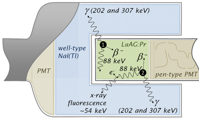
FIG. 3. A longitudinal section view of the experimental setup (not to scale). A LuAG:Pr scintillator coupled with a pen-type photomultiplier is fitted inside the well-type NaI(Tl) spectrometer. Two events of \beta detection by the LuAG:Pr in coincidence with the NaI(Tl) are schematically reported: (1) 202 + 307 keV are detected by the NaI(Tl) and the full 88 keV + \beta is detected by the LuAG:Pr; (2) again, 202 + 307 keV are detected by the NaI(Tl), the 88 keV generates a fluorescence x-ray (54 keV), which escapes the LuAG:Pr hence 88 - 54 = 34 keV + \beta is detected by the LuAG:Pr.
