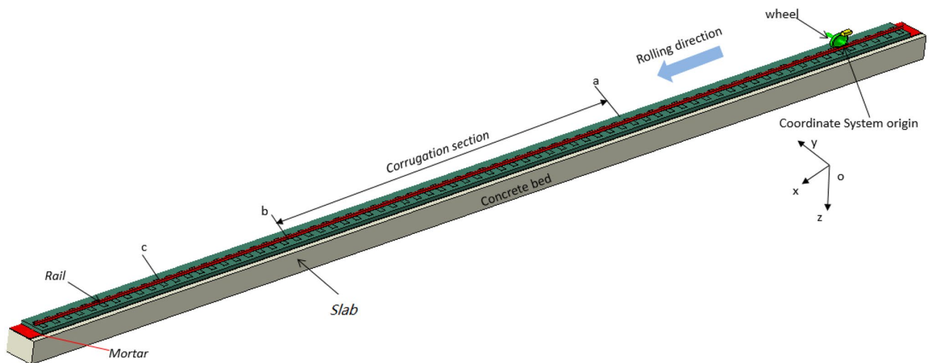
(a) Model overall view
